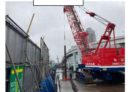
④UP14橋脚
